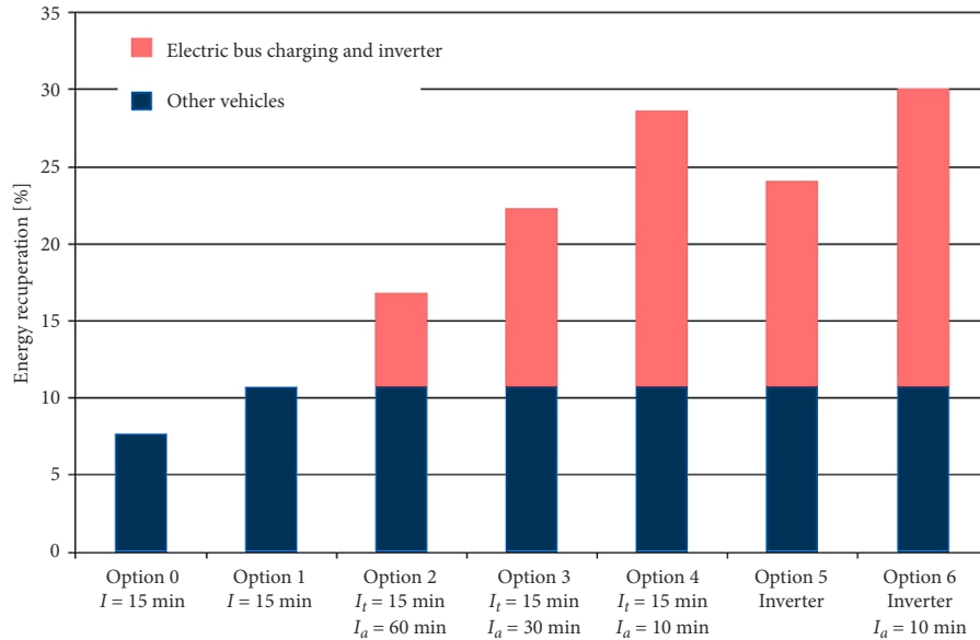
Figure 8. Comparison of energy recuperation in individual options analysed: blue colour – consumption of recuperation energy by other vehicles; red colour – increase of energy recuperation following the installation of electric bus charging point; I_t – frequency of trolleybus service; I_a – frequency of electric bus service (and charging); inverter – installation of the inverter, using the recovered energy for supply of public building facilities
