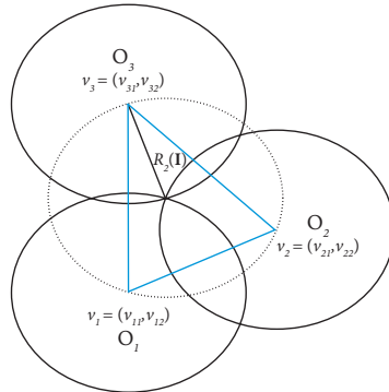
Fig. 1. Covering of a triangle (two-dimensional simplex) \mathbf{I} by disks (2-balls) O_i, i = 1, \dots, n + 1 of the same radius R_2(\mathbf{I})
