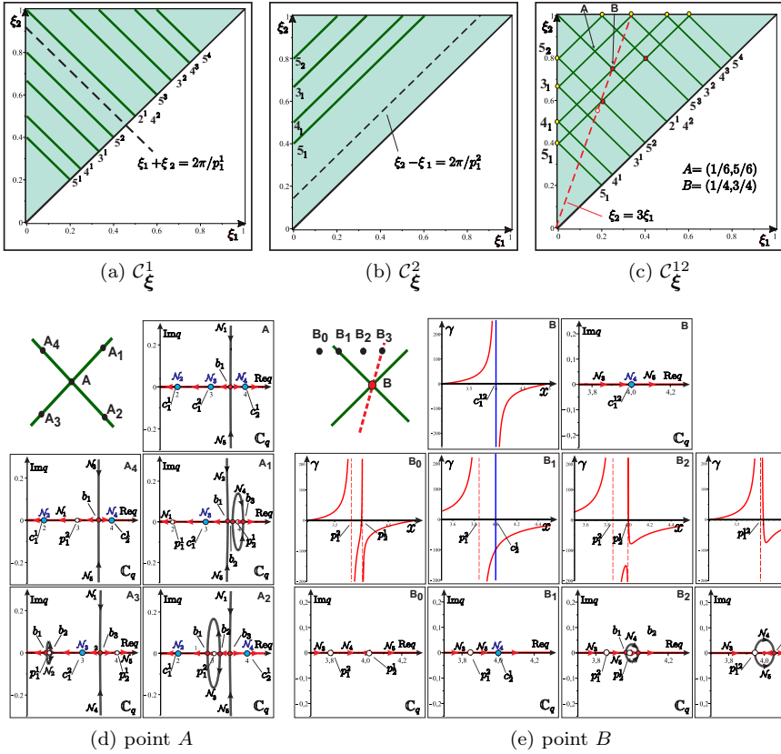
Figure 9. CE points ( c_k = \pi k, k = 1, \dots, 5 ) in Phase Space S_{\xi} and Spectrum Curves in the points A and B and in their neighbourhood.
